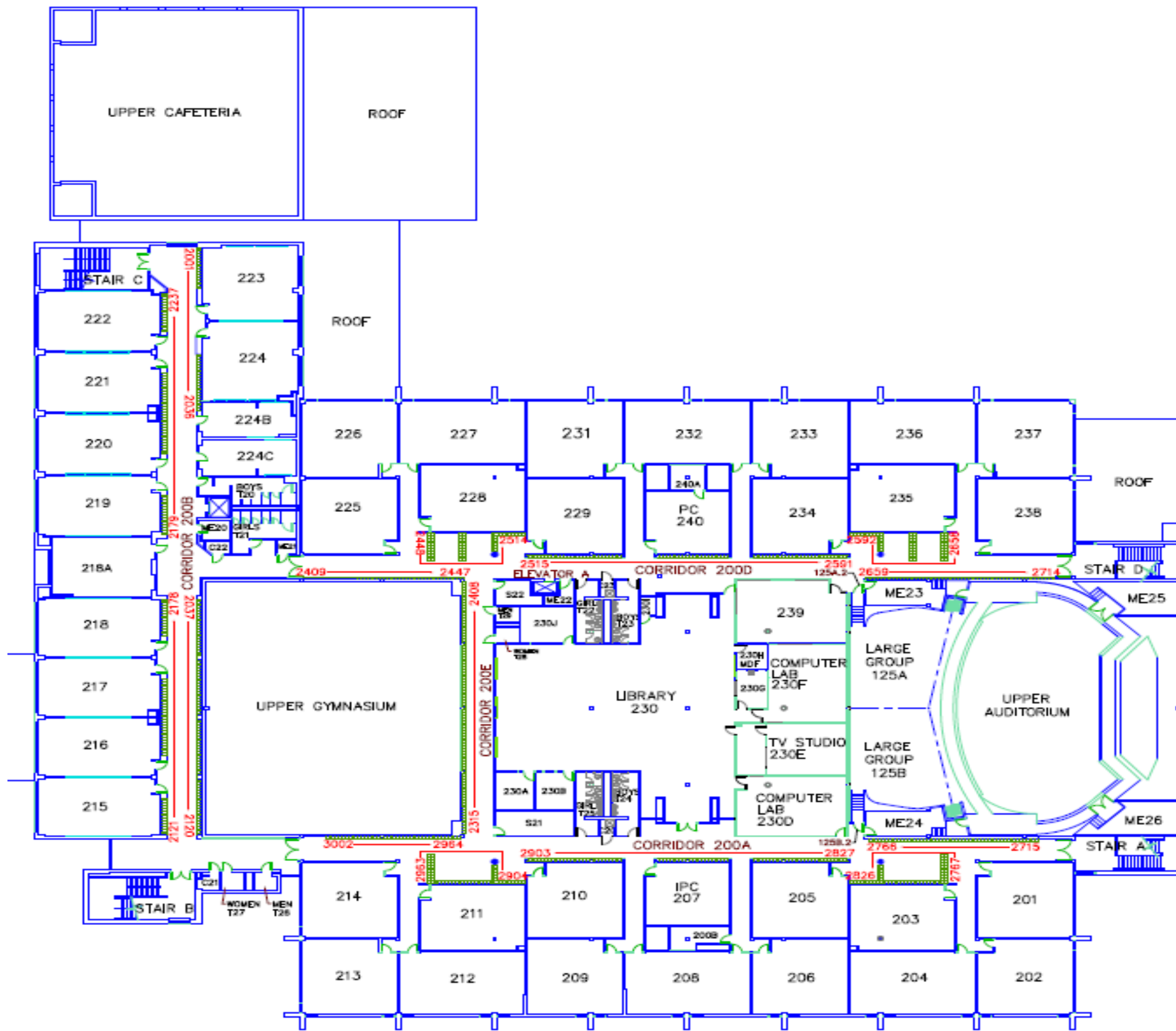
HOLICONG MIDDLE SCHOOL SECOND FLOOR PLAN
