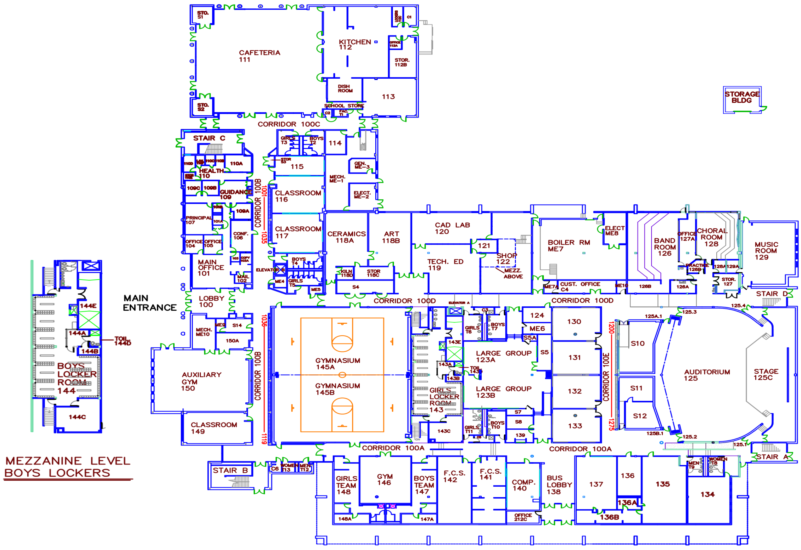
HOLICONG MIDDLE SCHOOL FIRST FLOOR PLAN
